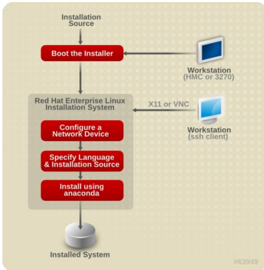
Figure 18.1. The Installation Process
