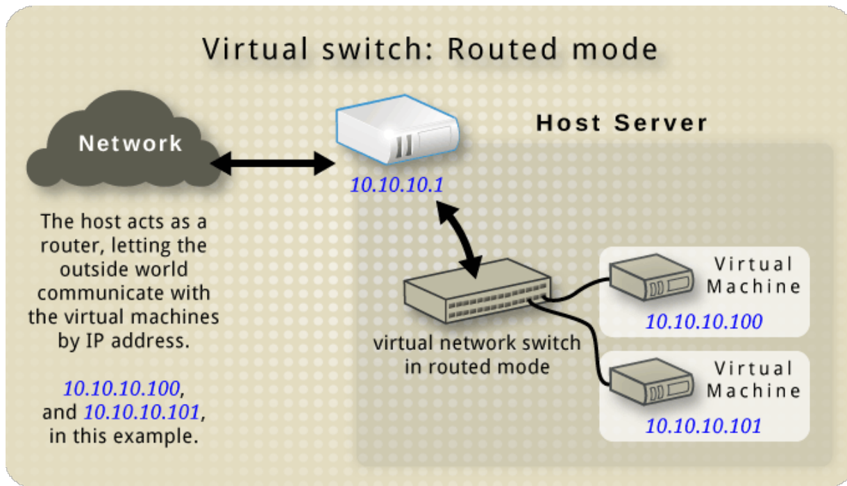
Figure 18.5. Virtual network switch in routed mode
