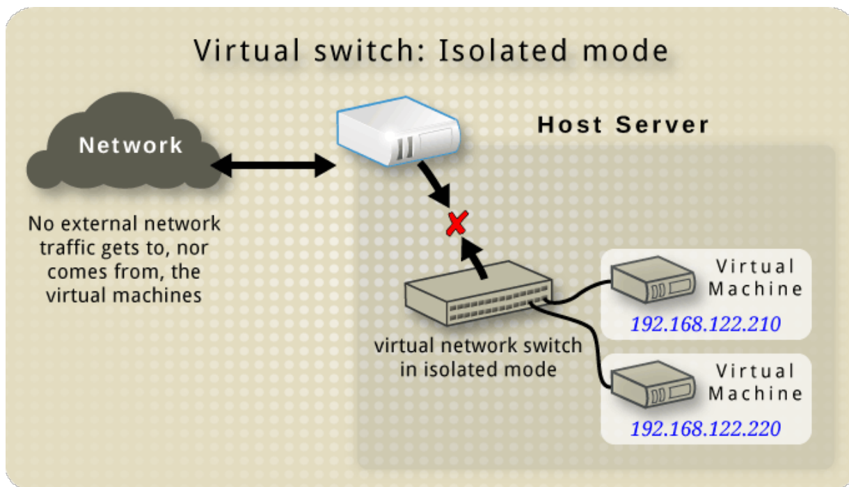
Figure 18.6. Virtual network switch in isolated mode
