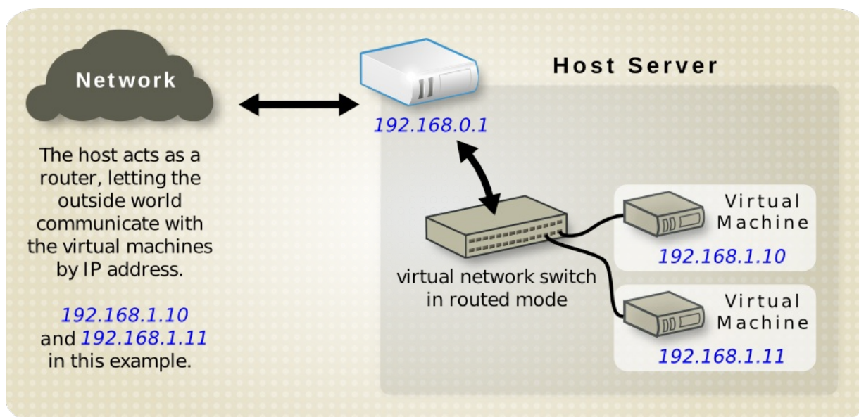
Figure 18.10. Virtual server using static IP addresses
