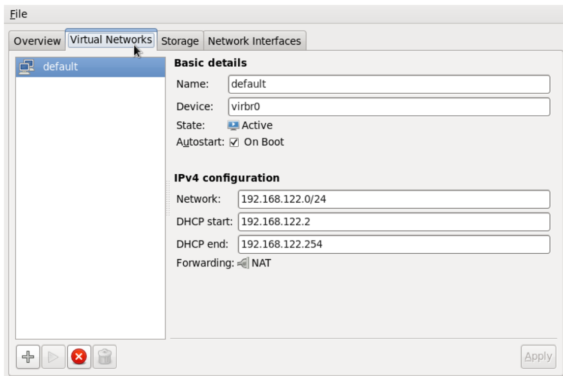
Figure 18.12. Virtual network configuration
