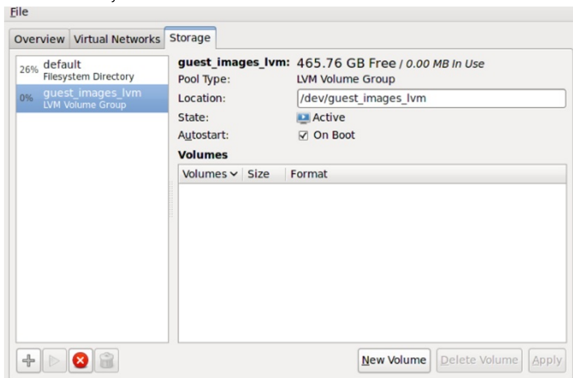
Figure 12.17. Confirm LVM storage pool details
