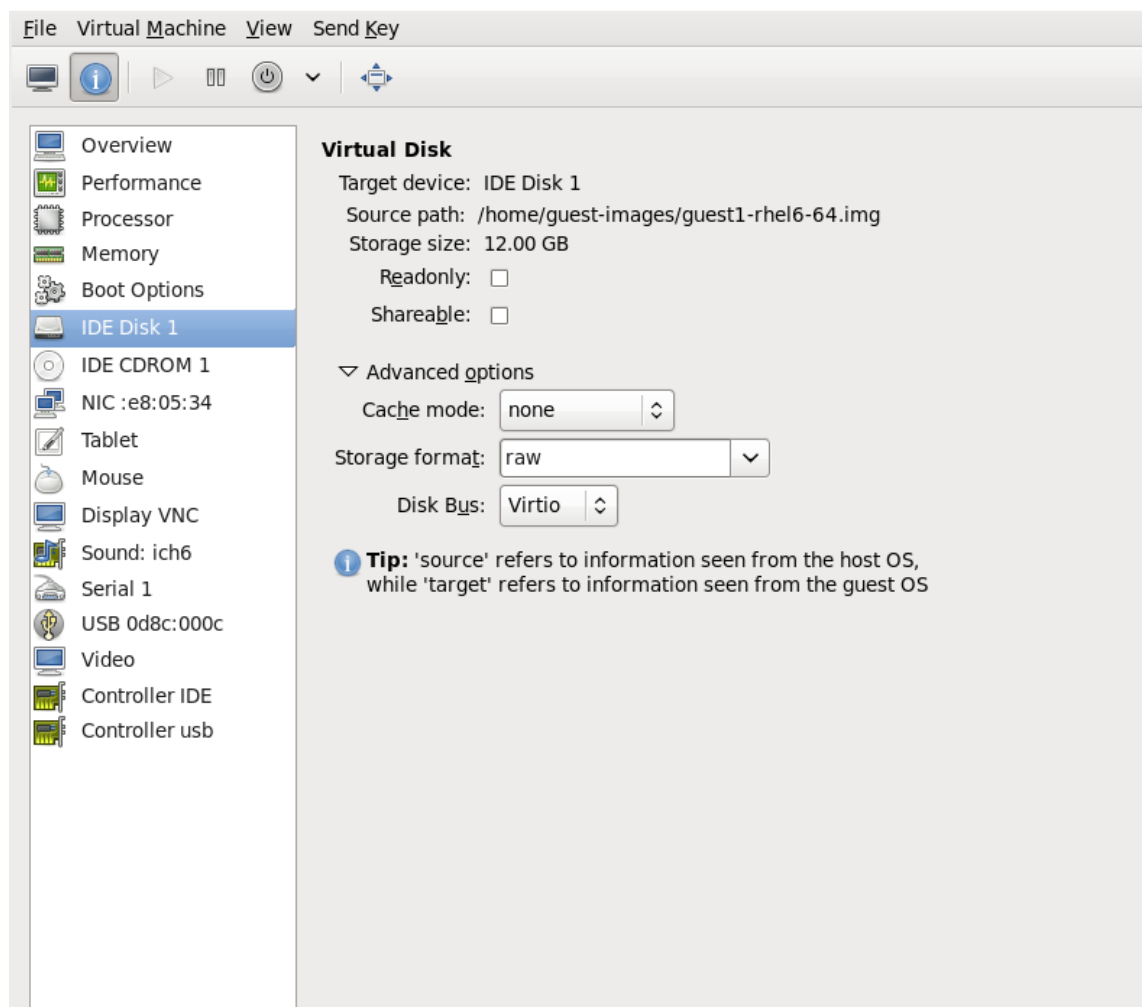
Figure 15.16. Displaying disk configuration
