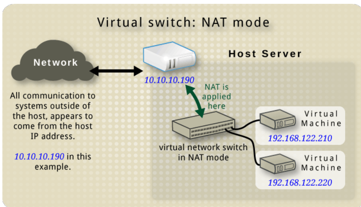
Figure 18.3. Virtual network switch using NAT with two guests
