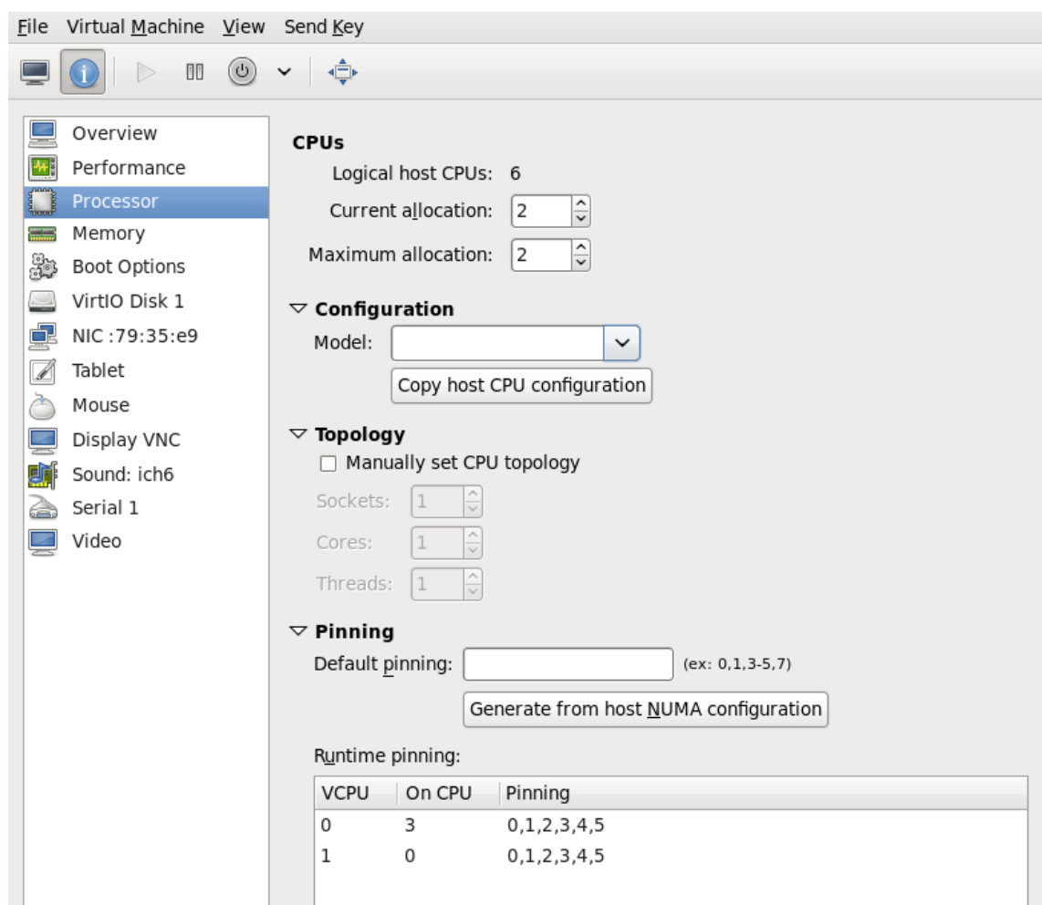
Figure 15.14. Processor allocation panel
