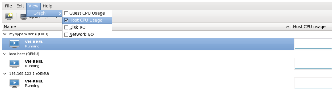
Figure 15.22. Enabling host CPU usage statistics graphing
