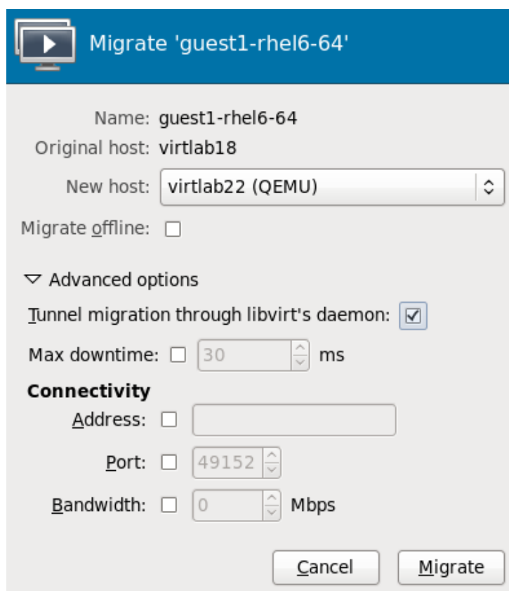
Figure 5.6. Choosing the destination host physical machine and starting the migration process
