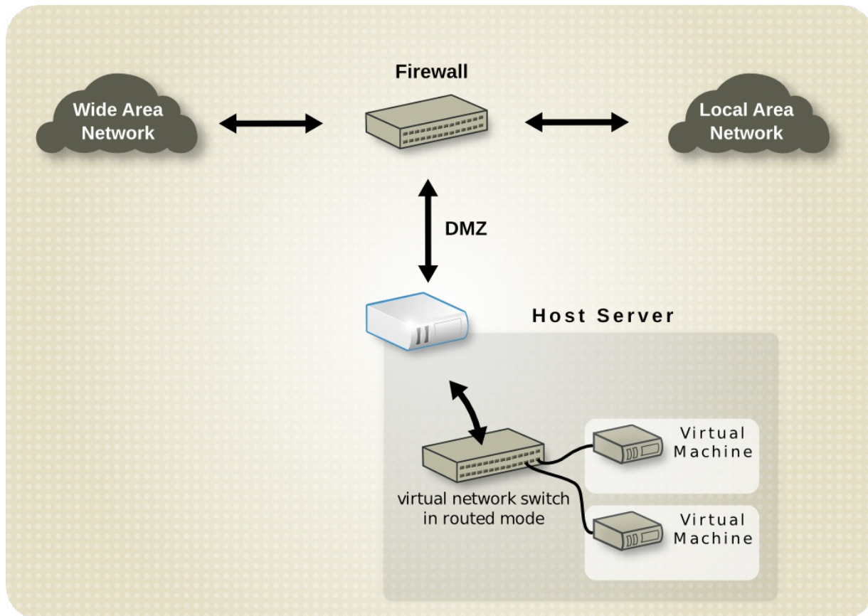
Figure 18.8. Sample DMZ configuration
