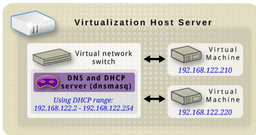
Figure 18.4. Virtual network switch running dnsmasq
