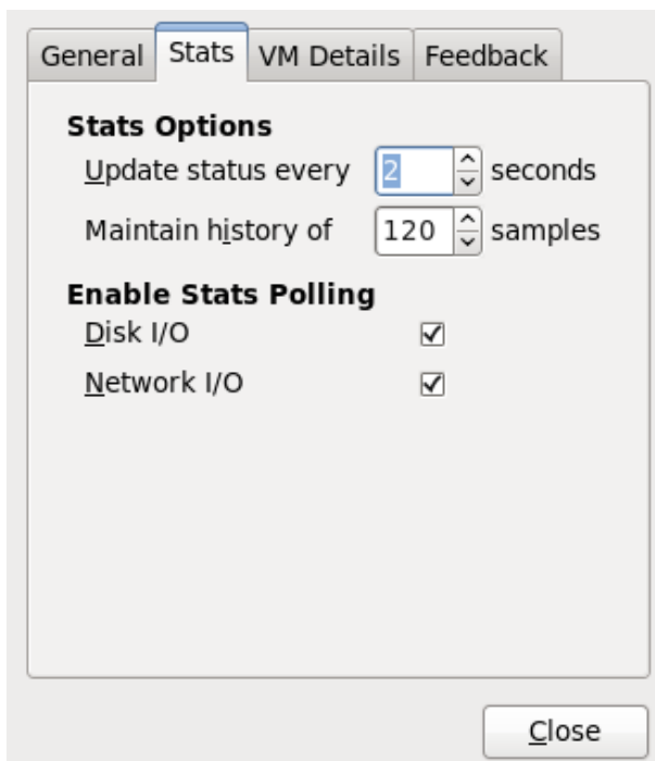
Figure 15.19. Configuring performance monitoring
