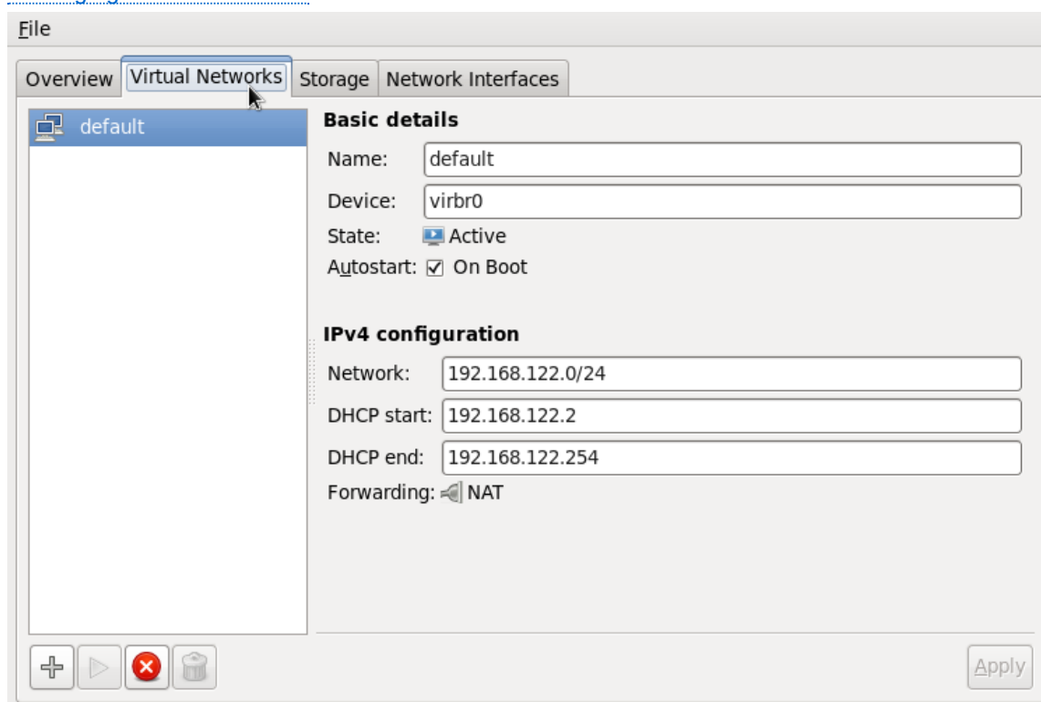
Figure 18.13. Virtual network configuration
