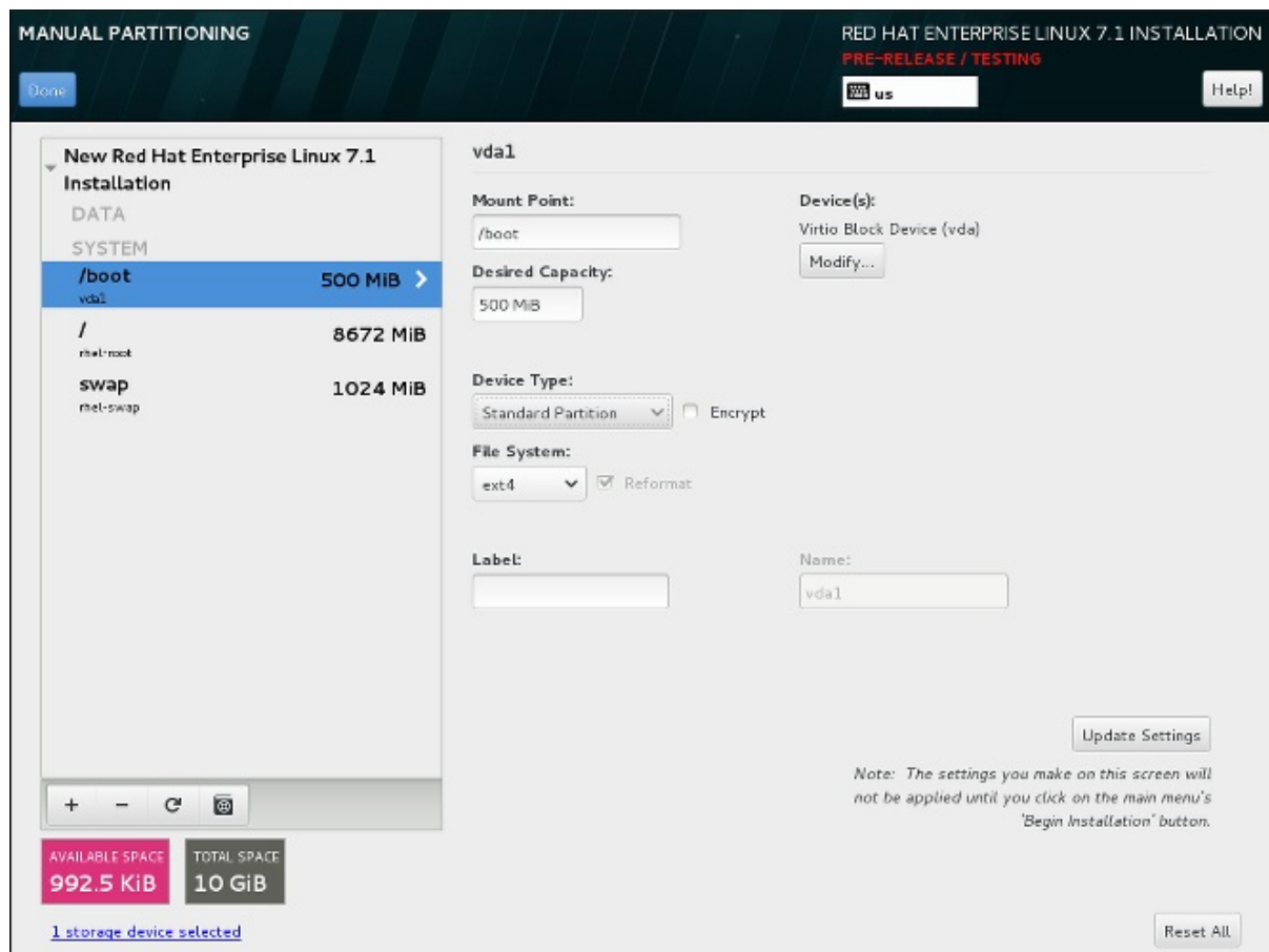
Figure 3.2. The redesigned Manual Partitioning screen
