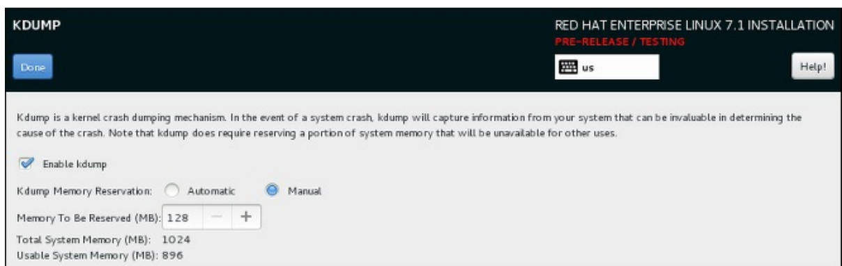
Figure 3.1. The new Kdump screen
