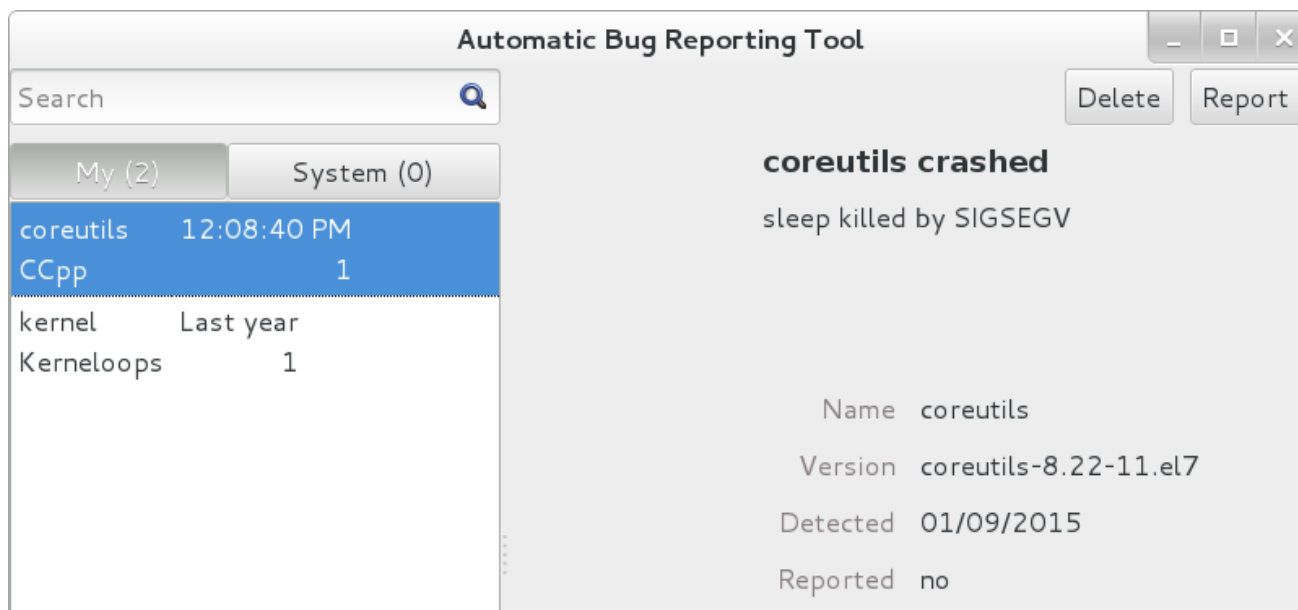
Figure 25.3. ABRT GUI
