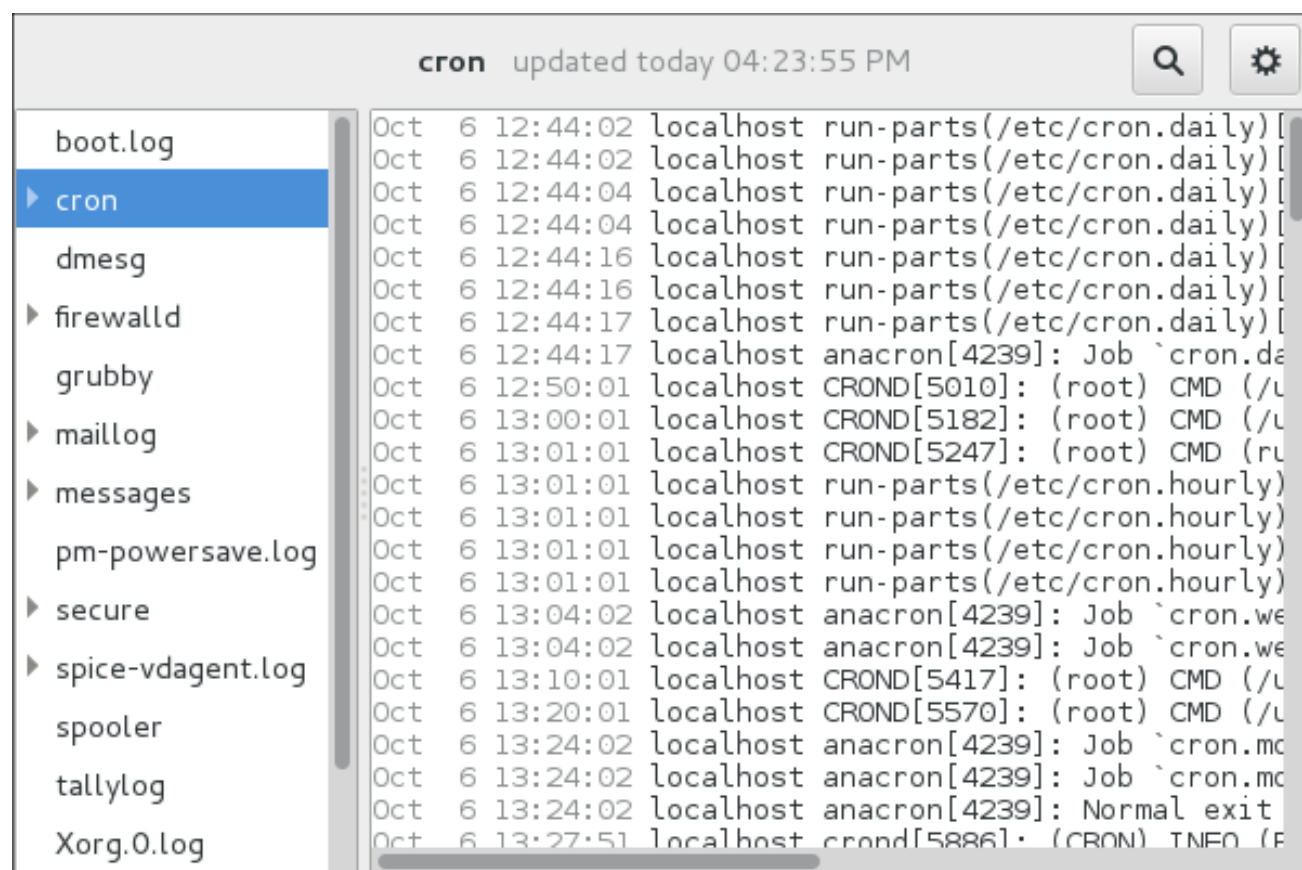
Figure 23.2. System Log
