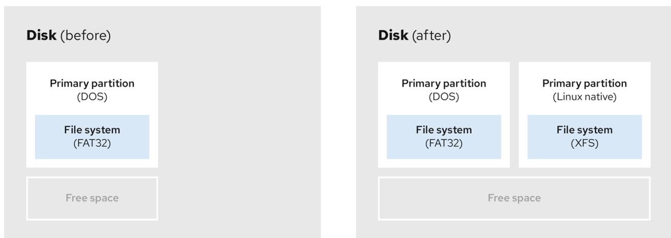
Figure 19.1. Disk with unpartitioned free space
